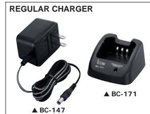
BC-171 DESKTOP CHARGER + BC-147 AC ADAPTER Charges the battery pack in 8–10 hours (approx.).
