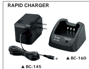
BC-160 DESKTOP CHARGER + BC-145 AC ADAPTER Charges the BP-232 in 3 hours (approx.). BC-119N + AD-106 + BC-145 is also available.
