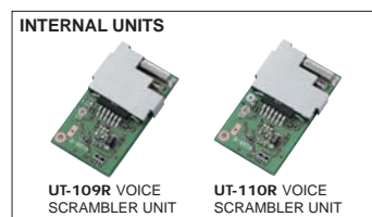
UT-109R : Up to 32 scrambling codes are available. 40-pin type. UT-110R : Up to 1020 scrambling codes are available. 40-pin type.
