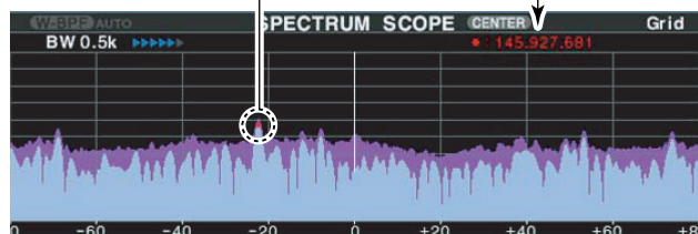
Peak indicator Peak frequency
