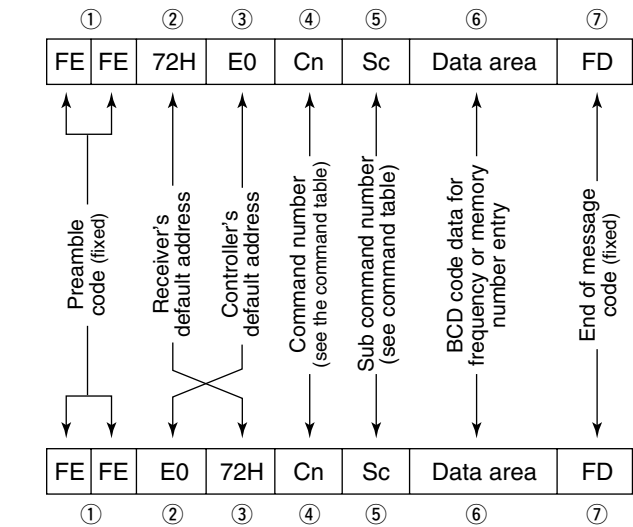
IC-R9500 to controller
