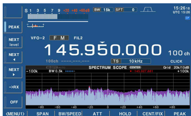
Peak indicator Peak frequency
